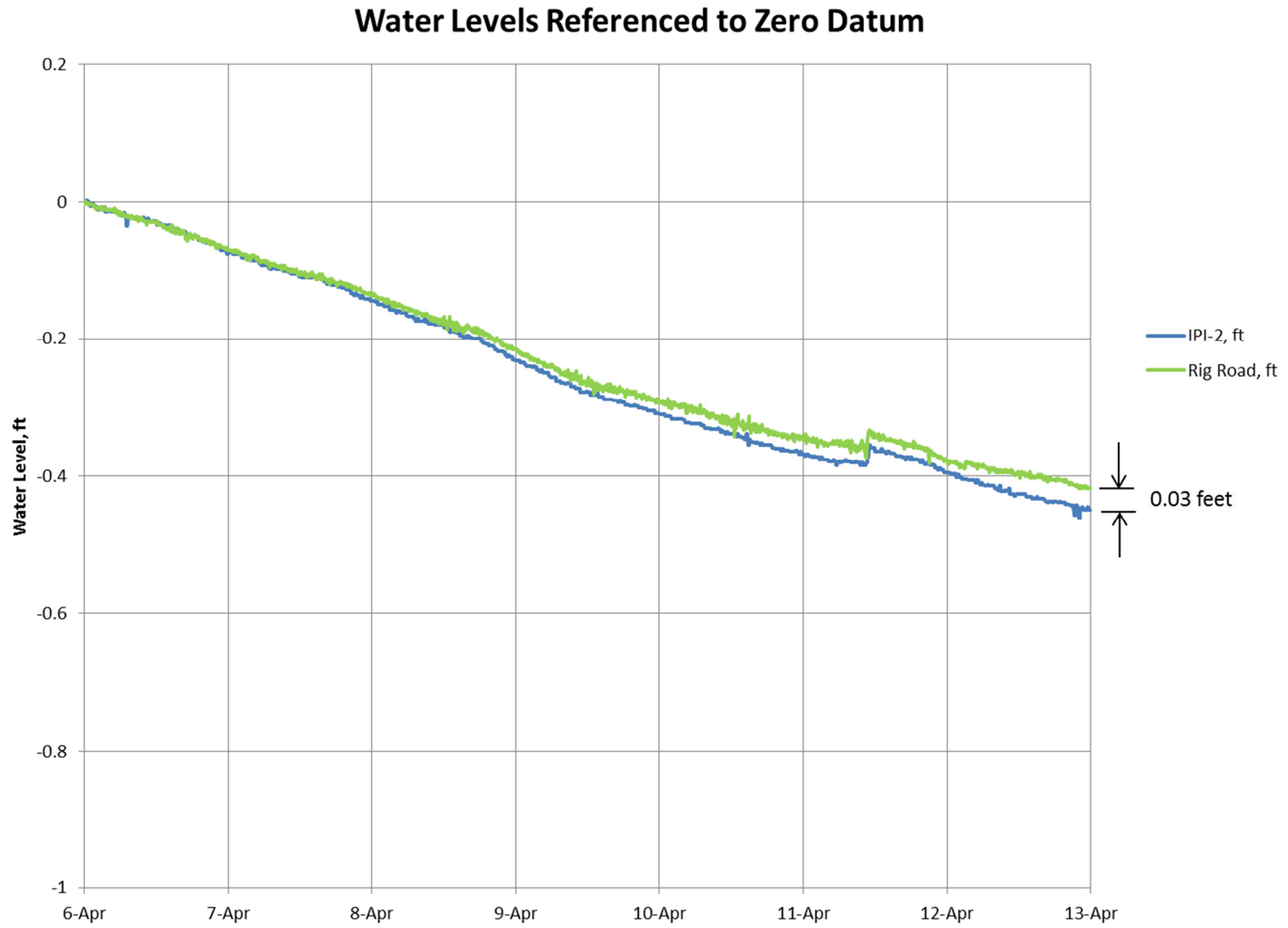
Figure 7. Water-Levels at IPI-2 and Rig Access Road Referenced to Zero Datum.
