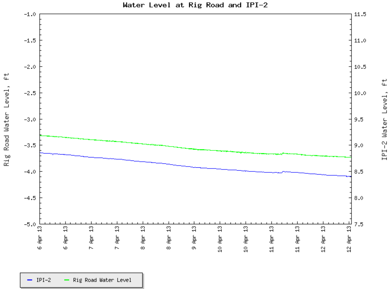
Figure 6. Water-Level Temporal Trends Showing Rig Access Road Data and IPI-2 Data.
