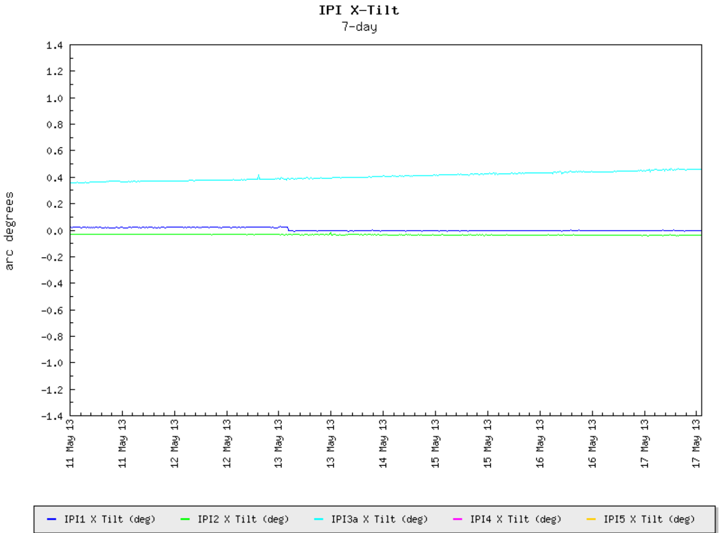
Figure 2. Inclinometer X-Direction Temporal Trends.
