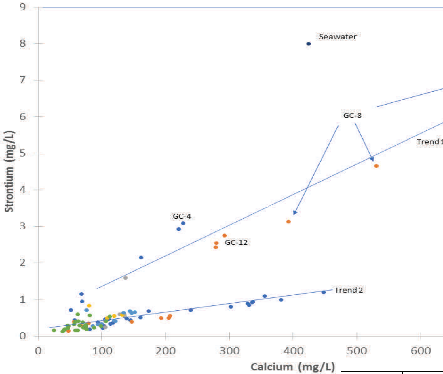
Figure 15. Strontium and calcium concentrations in groundwater in the vicinity of the Guidry Site. Source: Bruce K. Darling, Ph.D.
