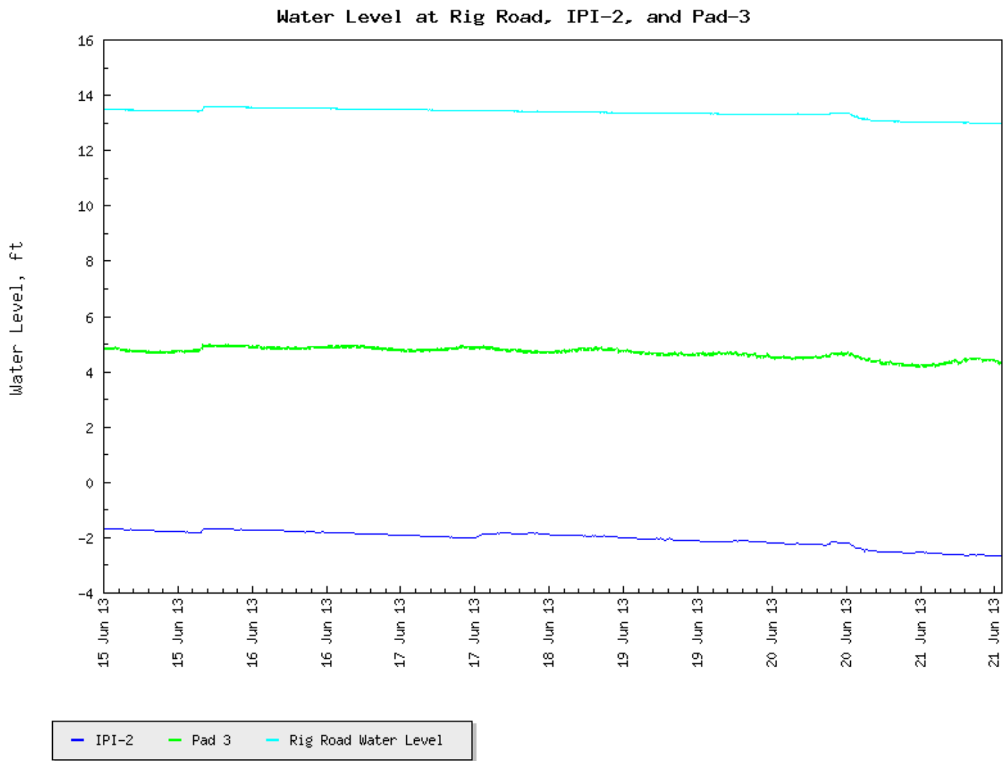
Figure 5. Water-Level Temporal Trends Showing Rig Access Road Data and IPI-2 Data (Water Levels Are Calibrated to Staff Gages at Each Site).
