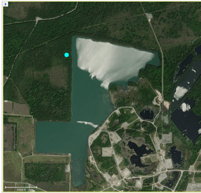
Figure 1. Left is an aerial image of Sulphur Mines salt area. The March 10, 2024 event location is show by cyan dot.
