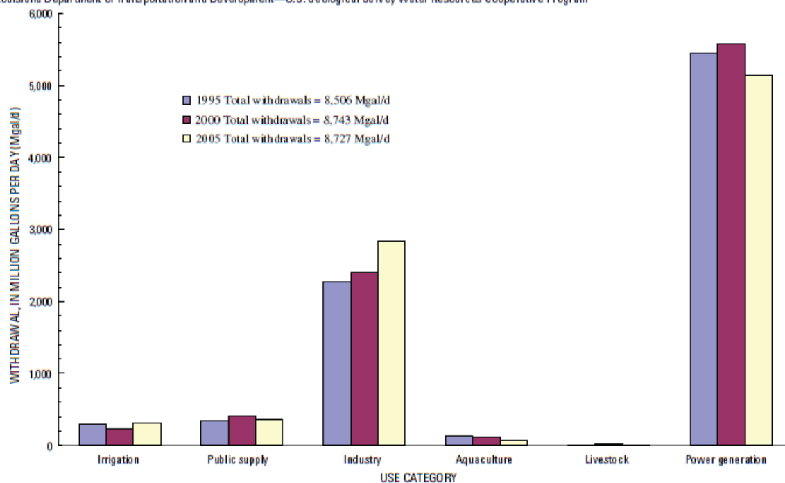
Figure 19. Surface-water withdrawals in Louisiana by use in 1995, 2000, and 2005 (J.K. Lovelace, written commun.; U.S. Geological Survey, 2006; Sargent, 2002; Sargent, 2007).
