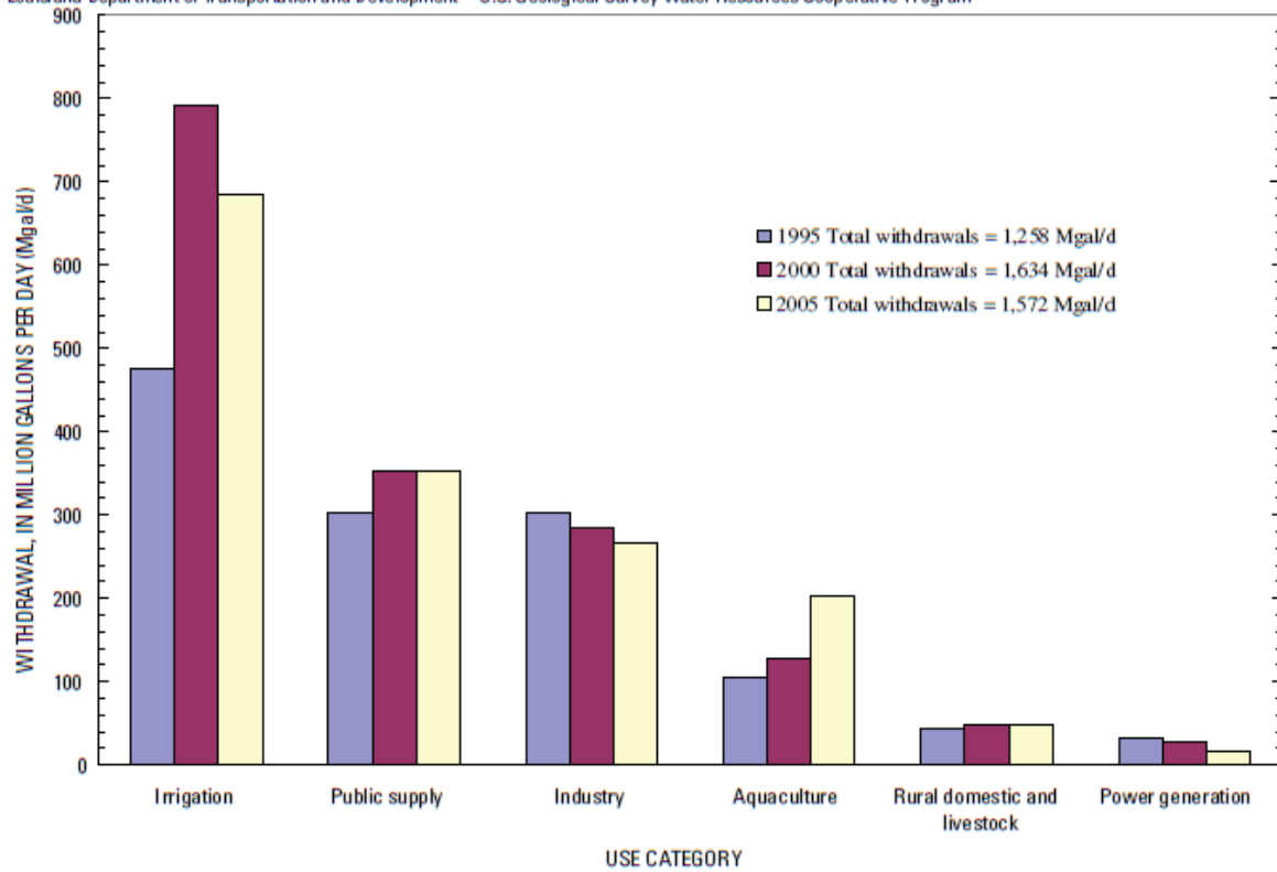
Figure 6. Ground-water withdrawals in Louisiana by use in 1995, 2000, and 2005 (J.K. Lovelace, written commun., U.S. Geological Survey, 2006; Sargent, 2002; Sargent, 2007).
