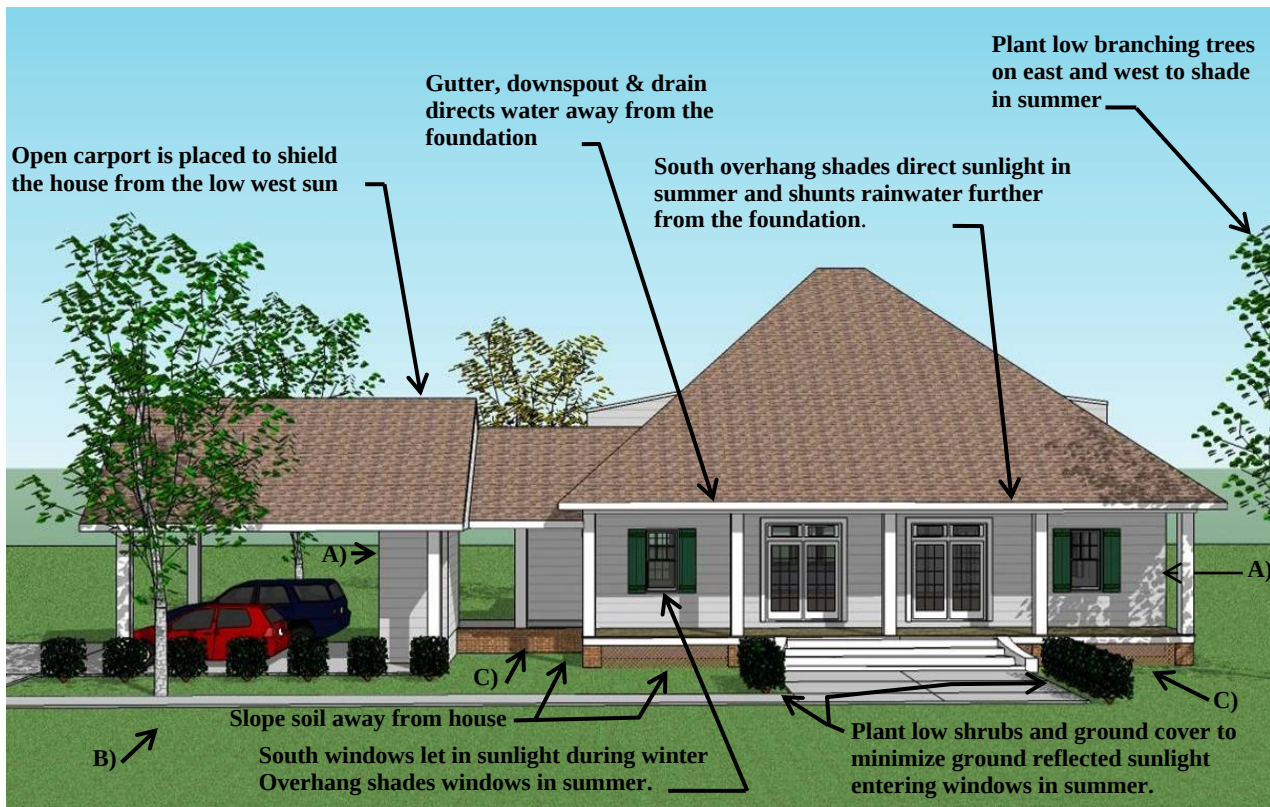
Figure 1-6 Site Planning
