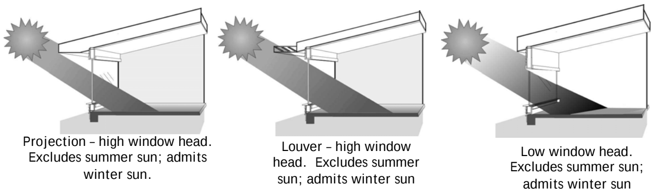
Figure 1-5 Overhang Types
