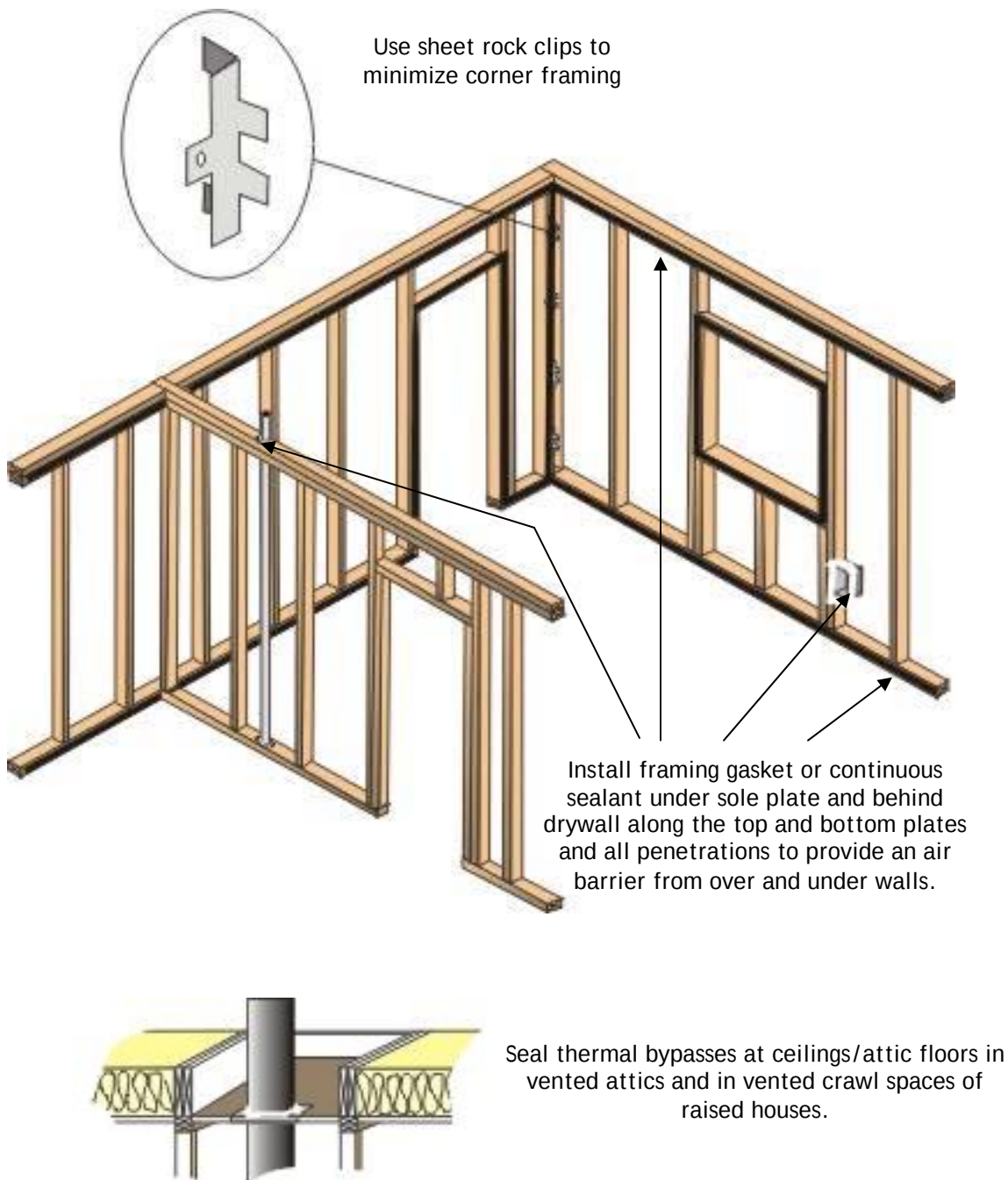
Figure 3-4 More Sealing Techniques
