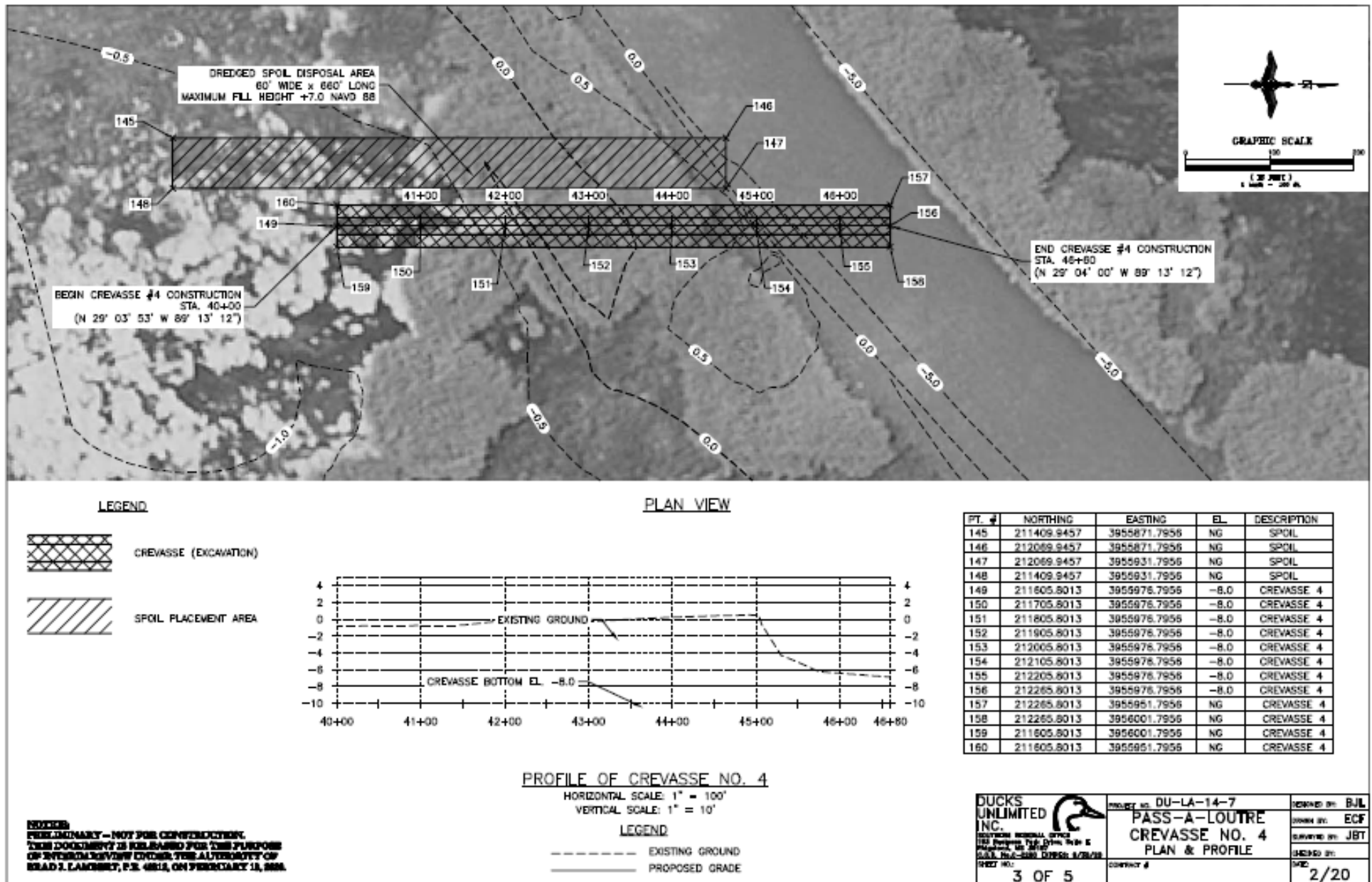
Figure 3. Plan and profile of crevasse excavation and spoil placement area.
